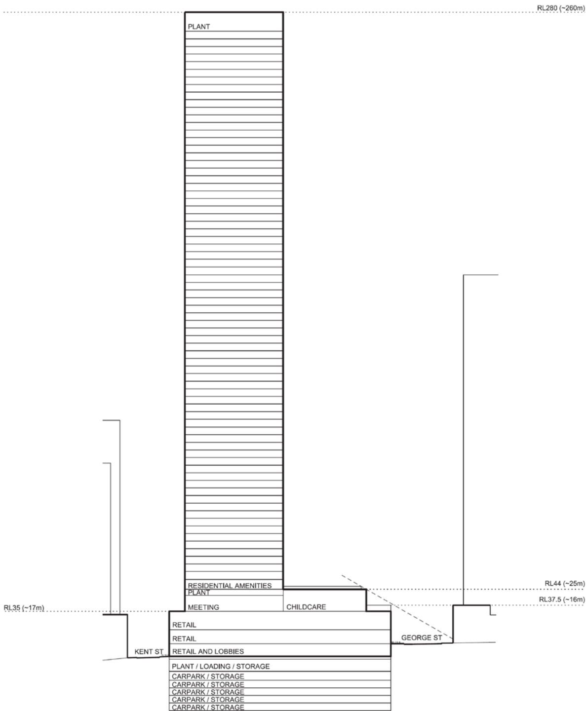
Figure 6.77 – Podium Design
